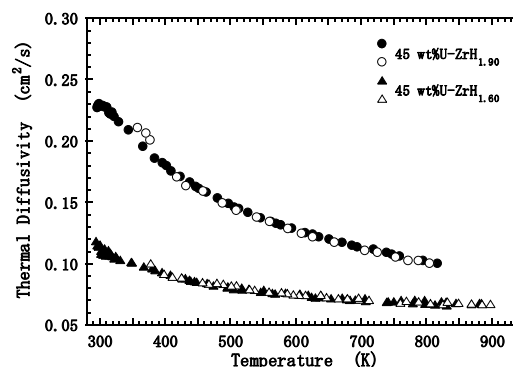
Fig. 2 Thermal diffusivities of \text{UZrH}_{1.6} and \text{UZrH}_{1.9} .
