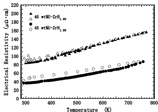
Fig. 3 Electrical resistivities of \text{UZrH}_{1.6} and \text{UZrH}_{1.9} .
