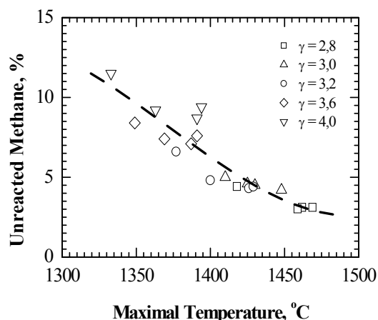
Fig. 4. Methane content in reaction products
