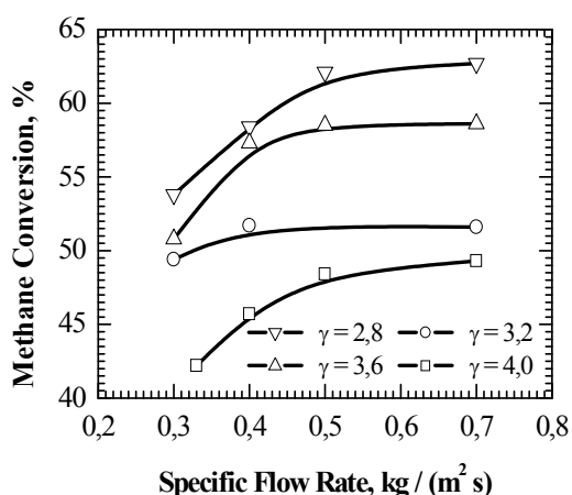
Fig. 3. Methane to hydrogen conversion factor
