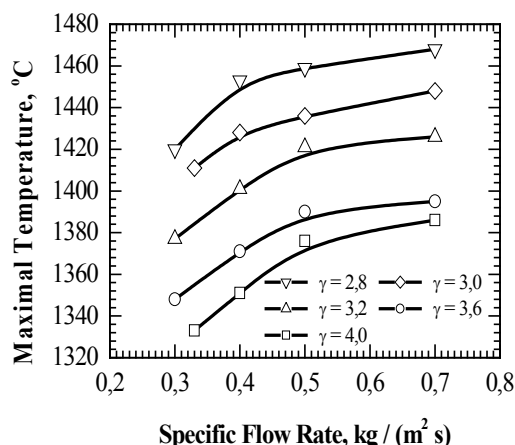
Fig. 2. The effect of equivalence ratio and mass flow rate on maximal temperature.
