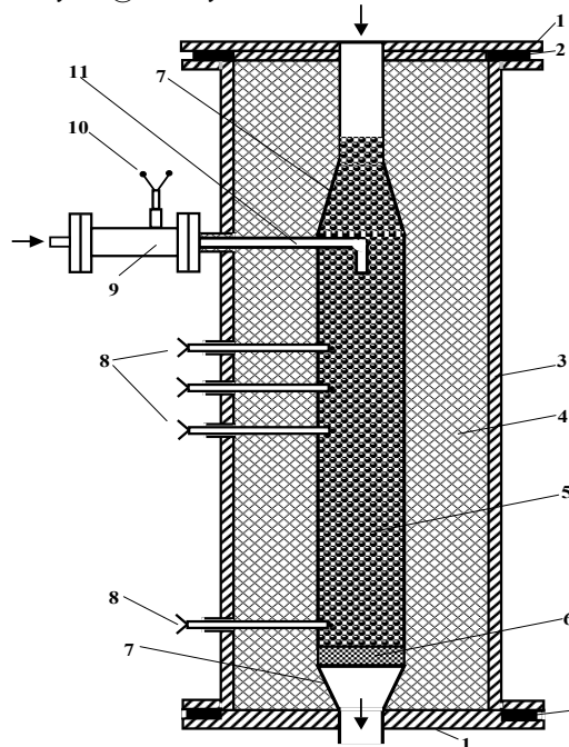
Fig. 1. Schematic of the experimental set-up. 1-flanges, 2-seal, 3-steel case, 4-high-temperature insulation, 5-ceramic bed, 6-porous ceramic disc, 7-quartz cone, 8-thermocouples, 9-preheat unit, 10-spark plug, 11-quartz tube.
